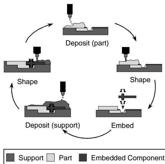
Figure 3.1 Shape Deposition Manufacturing consists of an alternating cycle of material deposition and shaping (in this case, machining). Prefabricated components can be embedded in mid-cycle.
