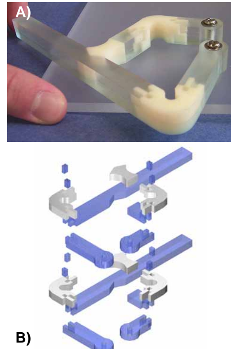
Figure 3.3 a) Prototype five-bar linkage with heterogeneous material properties, in which three of the joints have been replaced with flexures of a soft grade of plastic. b) Sequential order of layers for the linkage.
