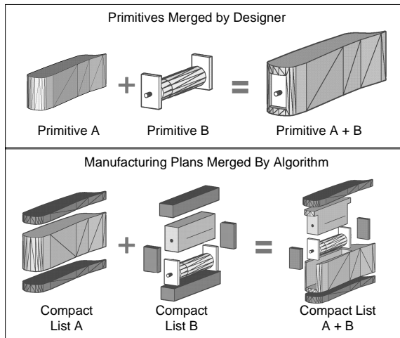
Figure 4.1 Design-by-Composition Interface. Here, designers compose designs from a library of “primitives.” Meanwhile, the design interface merges the individual process plans for each primitive into a combined process plan.
