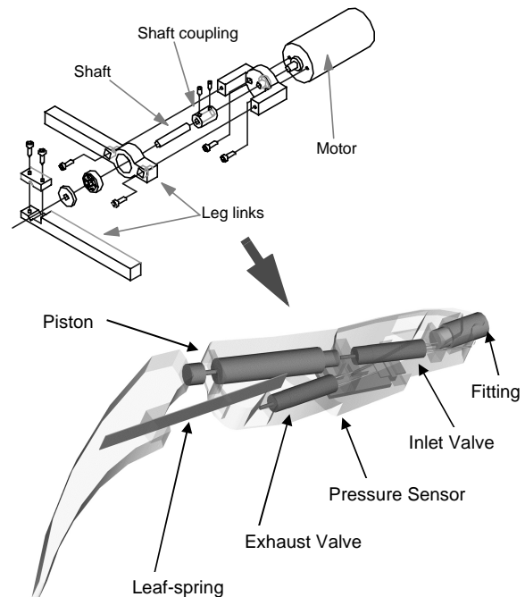
Figure 1.1 In the conventional approach, connecting a motor to a leg mechanism requires many small components and fasteners. In a leg built by Shape Deposition Manufacturing, parts are encapsulated in structural materials.
