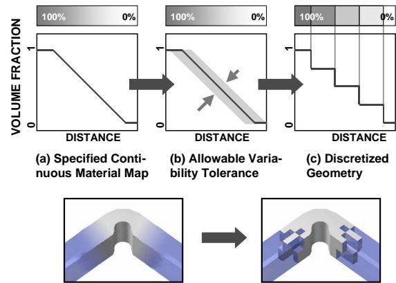
Figure 3.5. Constraints in the manufacturing process may require a discretization of the desired material property.
