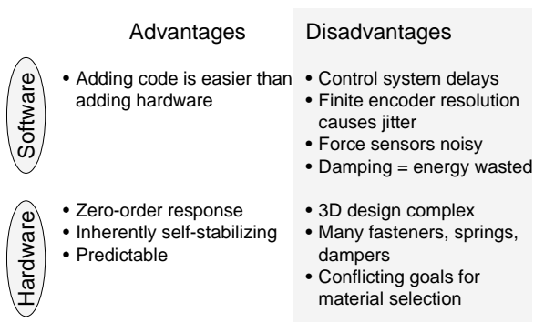
Figure 2.4 Despite the obvious advantages of implementing tuned impedance in hardware, the difficulties encountered in manufacturing preclude this option in favor of software implementation. However, software impedance control introduces a new set of concerns.
